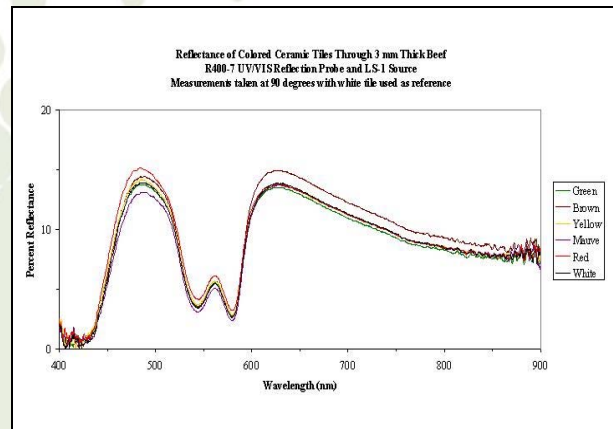
Figure 4: Reflectance of colored tiles through 3.0 mm thick fatty beef slices
