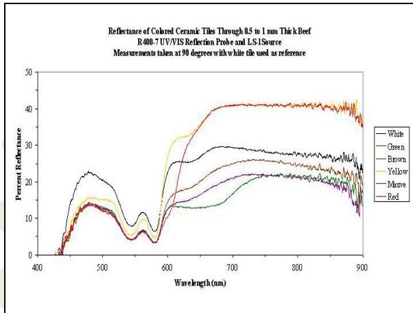
Figure 3: Reflectance of colored tiles through 0.5 to 1.0 mm thick beef slices
