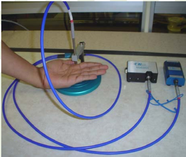
Figure 1: Proposed Experimental Set-up
