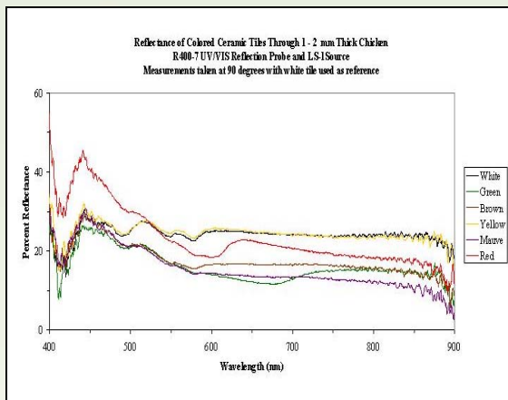
Figure 6: Reflectance of colored tiles through 1.0-2.0 mm thick chicken slices
