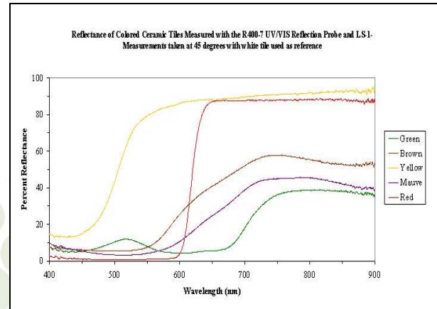
Figure 2: Reflectance of colored tiles obtained at 45 degrees
